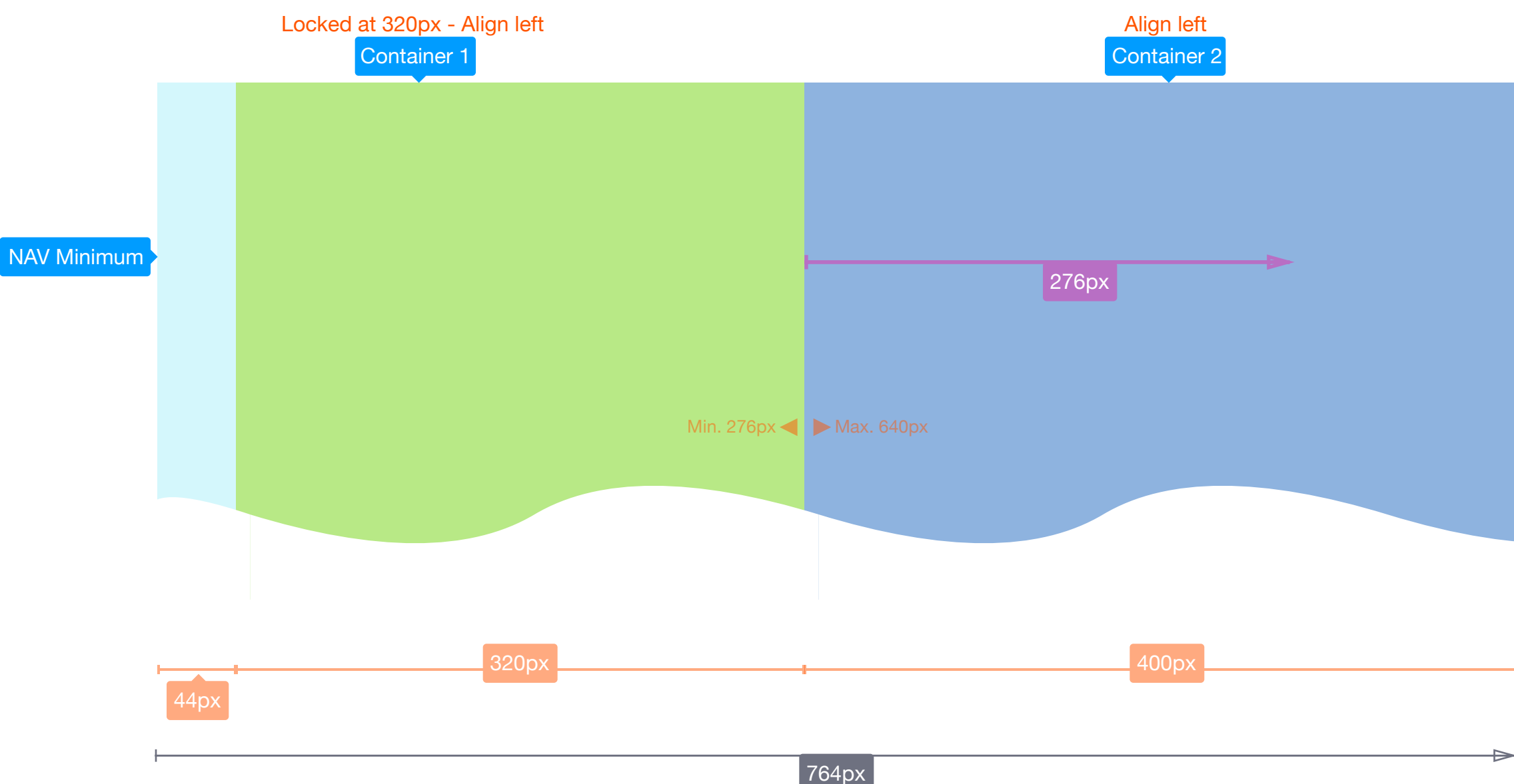
Screen width 640px - 1004px - Container 1, Container 2 are visible
