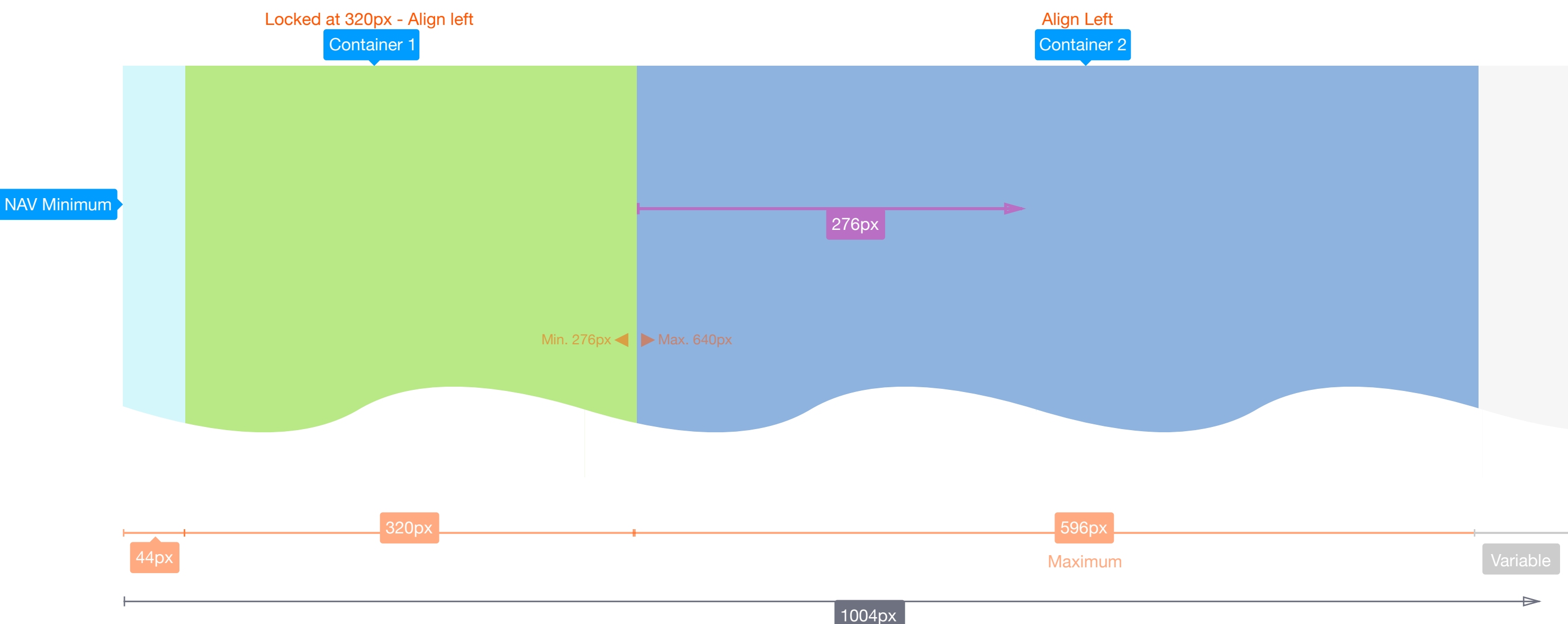
Screen width 640px - 1004px - Container 1, Container 2 are visible
