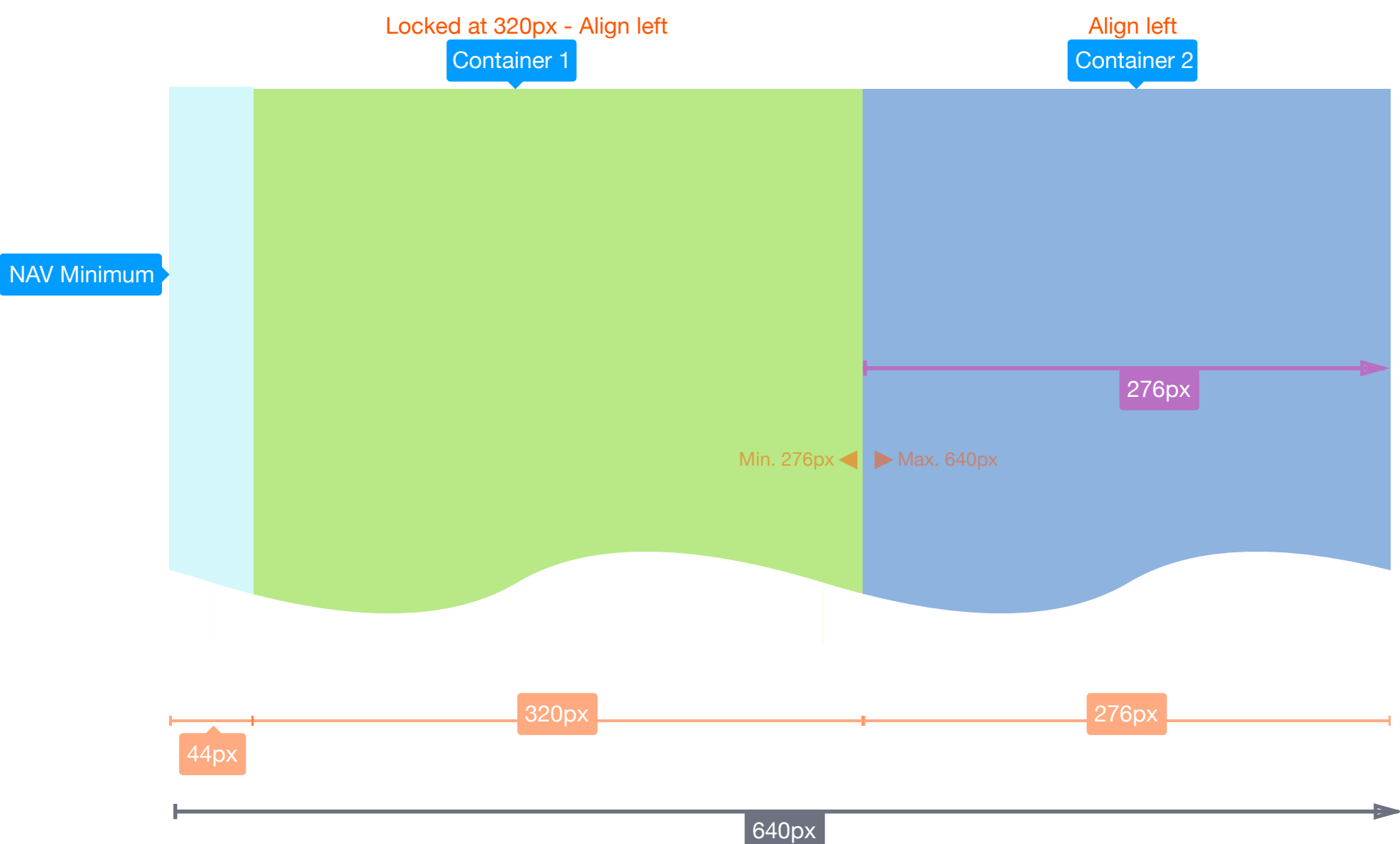
Screen width 640px - 1004px - Container 1 and Container 2, Nav Minimum visible
